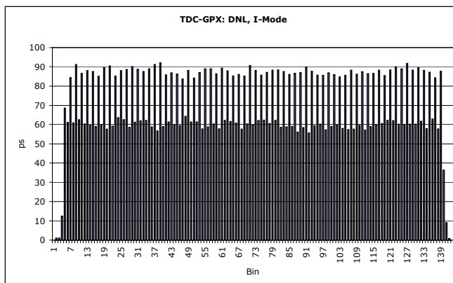
Figure 22: DNL
